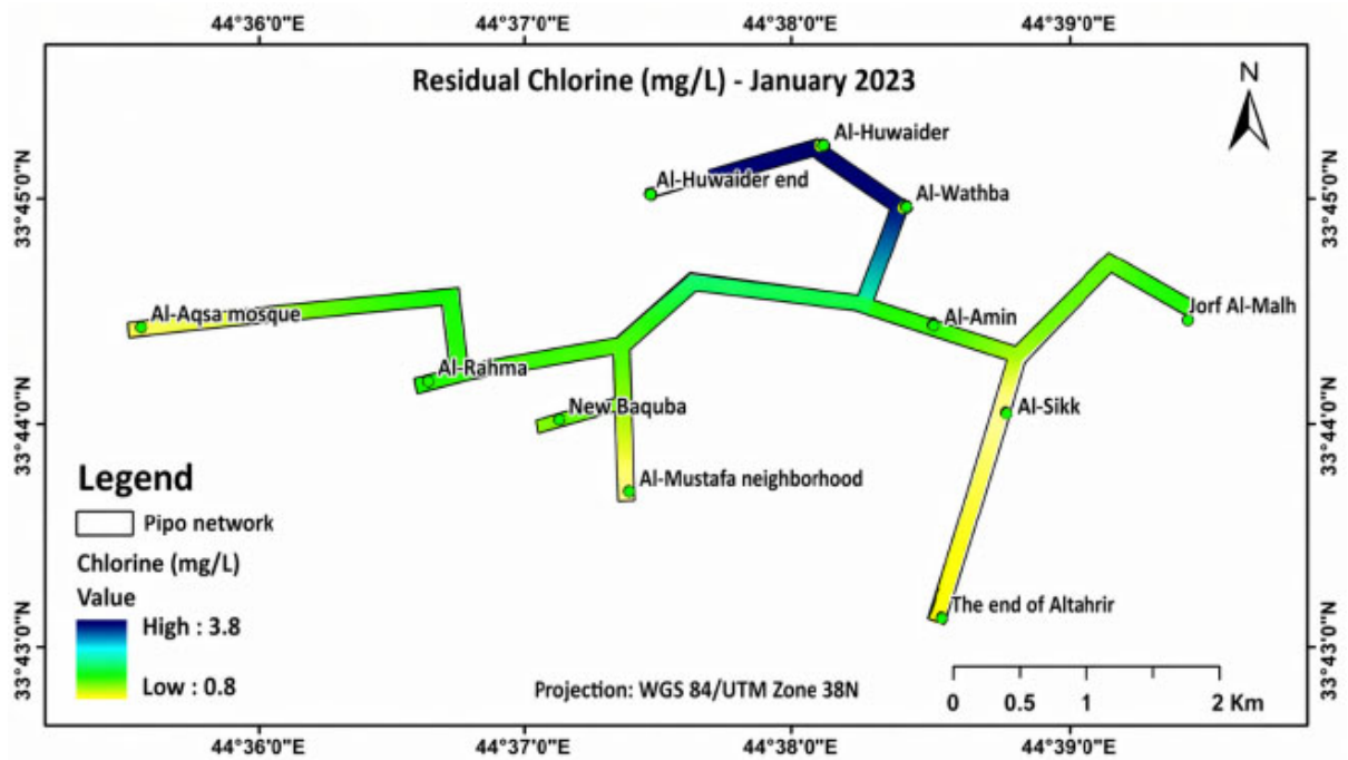
Fig. (9). Intensity of residual chlorine concentration of five selected lines using GIS program during January 2023.
