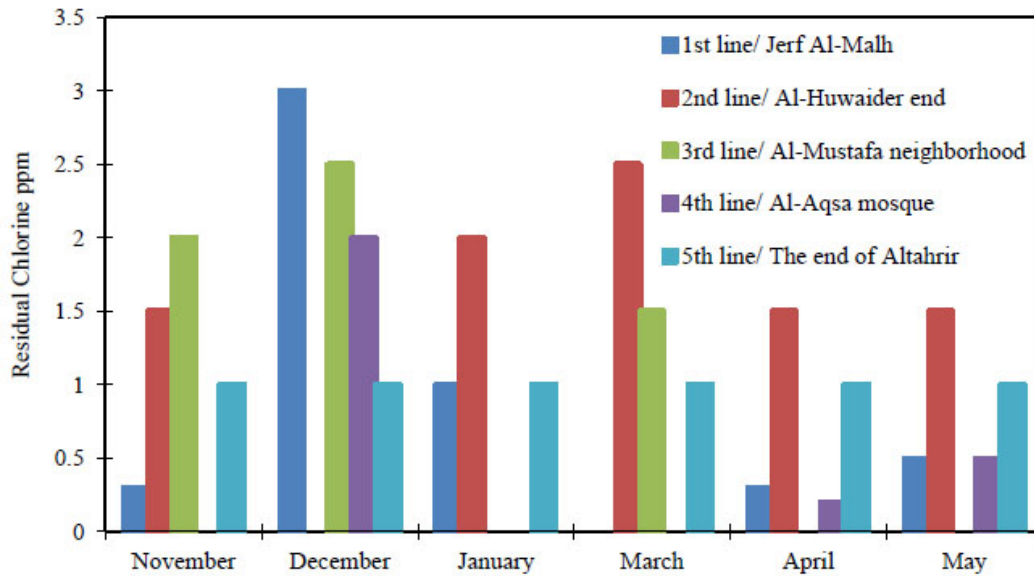
Fig. (6). Residual chlorine in water samples collected from the five selected lines.
