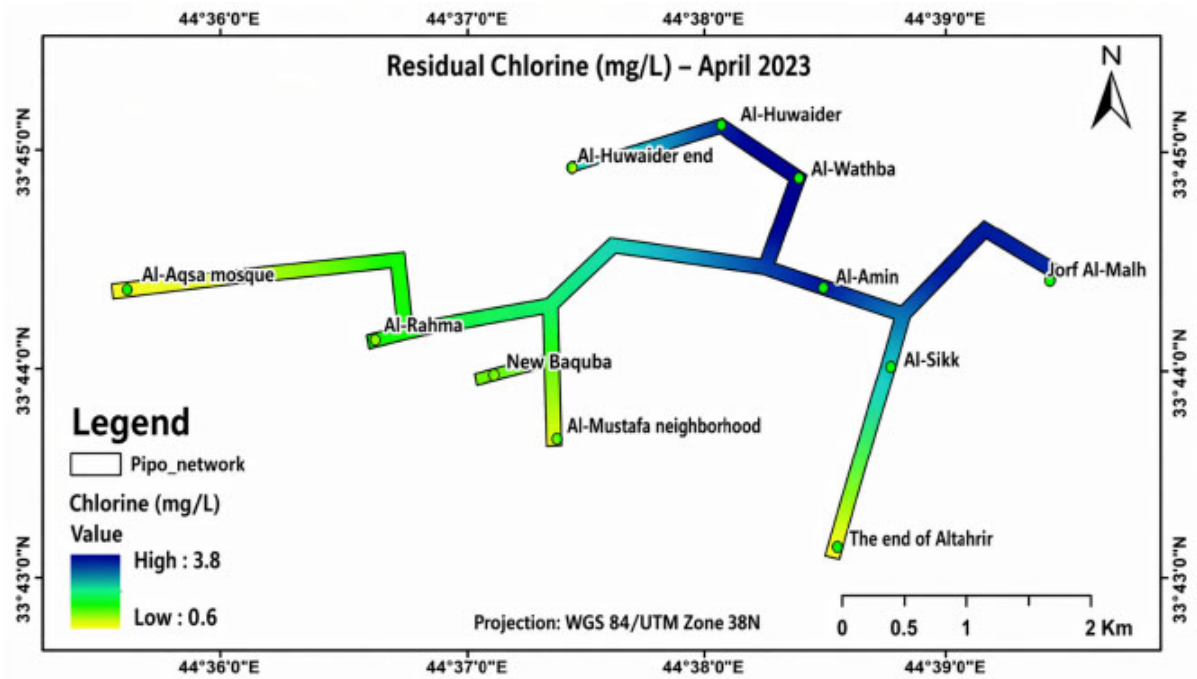
Fig. (11). Intensity of residual chlorine concentration of five selected lines using GIS program during April 2023.
