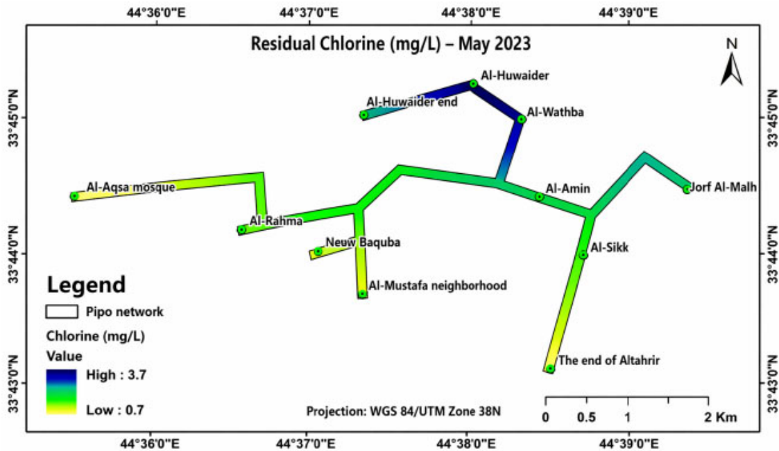
Fig. (12). Intensity of residual chlorine concentration of five selected lines using GIS program during May 2023.
