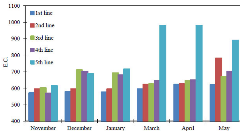
Fig. (5). Electrical conductivity of water samples collected from the five lines.
