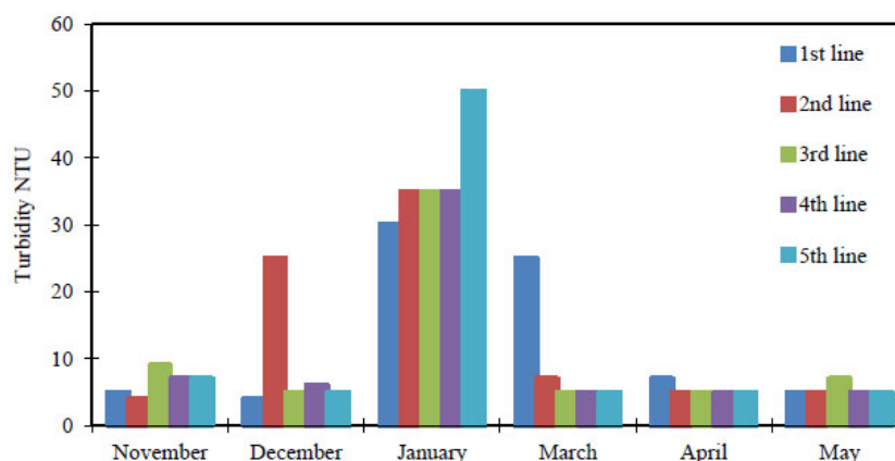
Fig. (4). Turbidity of water samples collected from the five selected lines.
