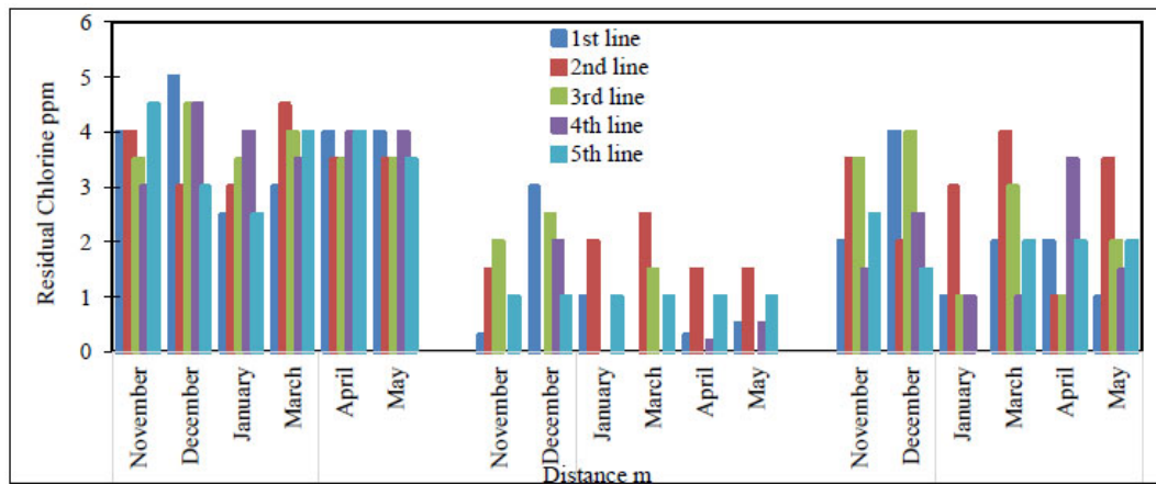
Fig. (13). Effect of distance on the residual chlorine of water samples collected from the five selected lines.
