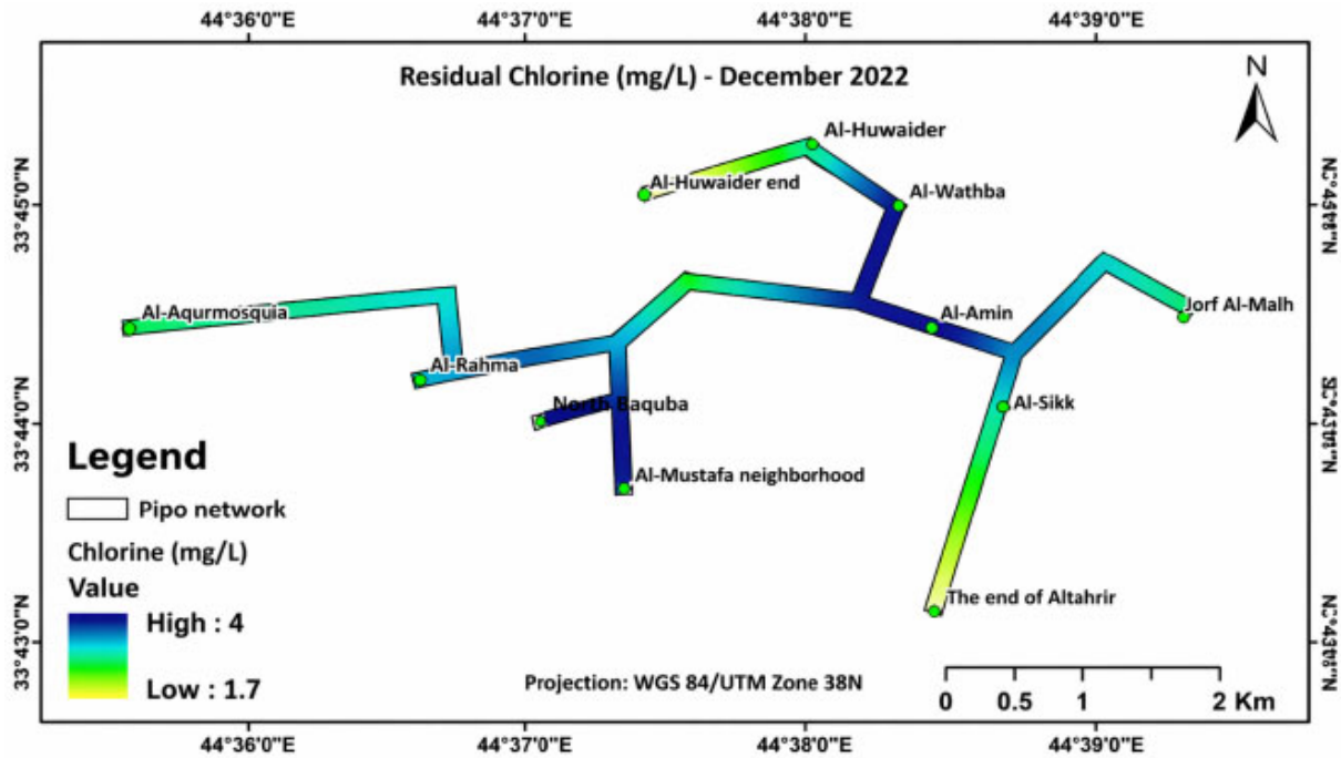
Fig. (8). Intensity of residual chlorine concentration of five selected lines using GIS program during December 2022.
