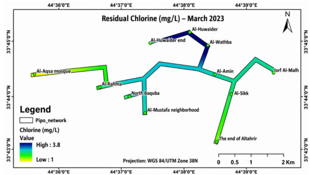
Fig. (10). Intensity of residual chlorine concentration of five selected lines using GIS program during March 2023.
