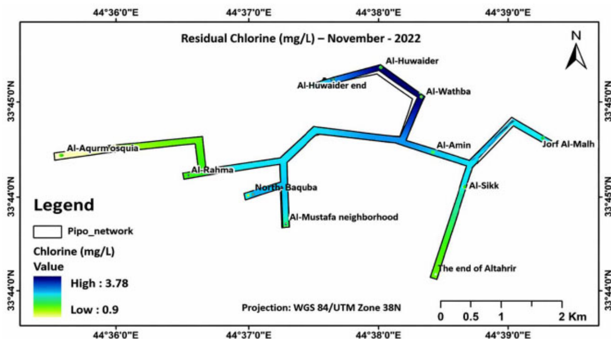
Fig. (7). Intensity of residual chlorine concentration of five selected lines using GIS program during November 2022.
