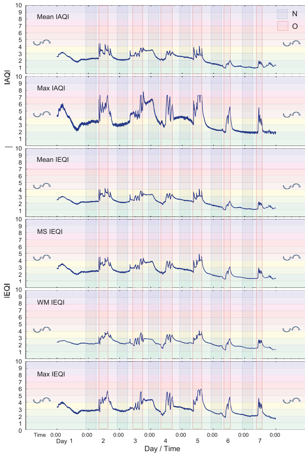
Fig. (3). Time series of the mean Indoor Air Quality Index (Mean IAQI), Maximal Indoor Air Quality Index (Max IAQI), Mean Indoor Environment Quality Index (Mean IEQI), root Mean Square Indoor Environment Quality Index (MS IEQI), weighted mean square indoor environment quality. index (WM IEQI) and maximal indoor environment quality index (Max IEQI) in the classroom. N - nighttime, O - occupied by students.
